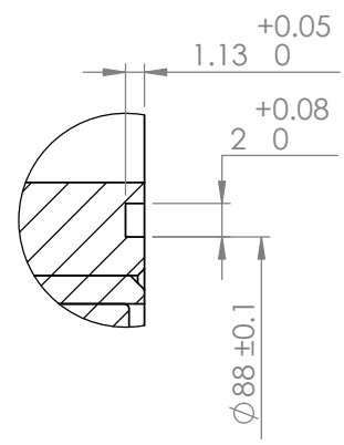
DETAIL A O-RING GLAND SCALE 2:1
