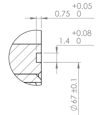
DETAIL A O-RING GLAND SCALE 3 : 1
