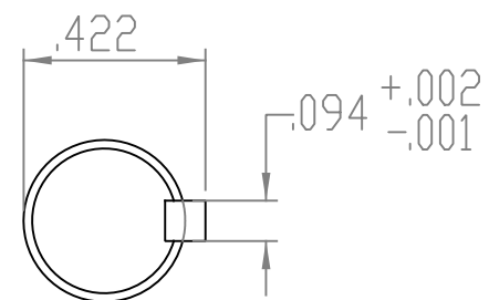
KEY DETAIL SCALE 2 : 1
